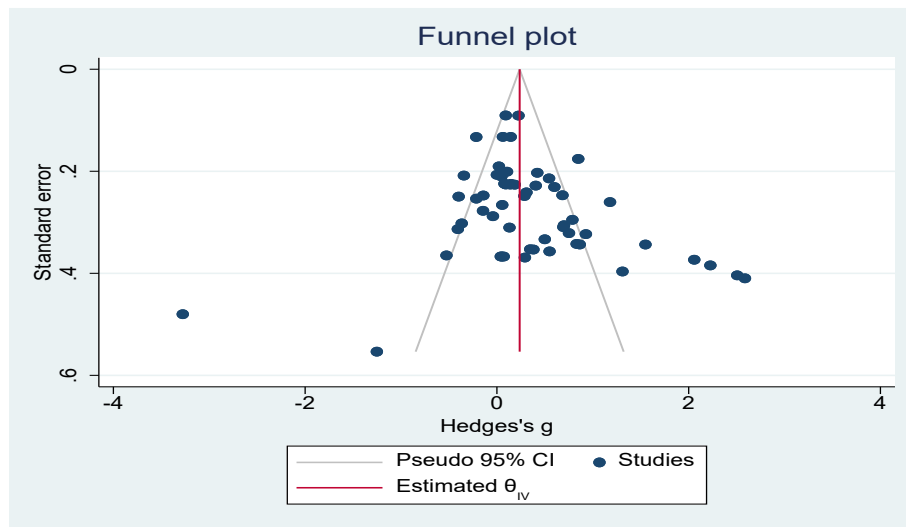
Funnel plot of interventions.
